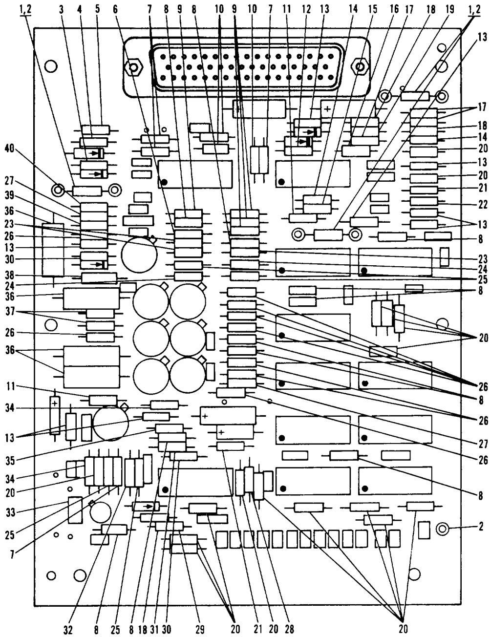
Figure 40. +5V Inverter/Driver Circuit Card subassembly (Sheet 1 of 2)
