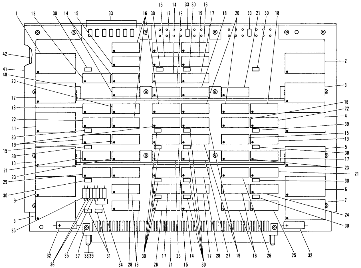
Figure 2. Type 7ABL Circuit Card Assembly
