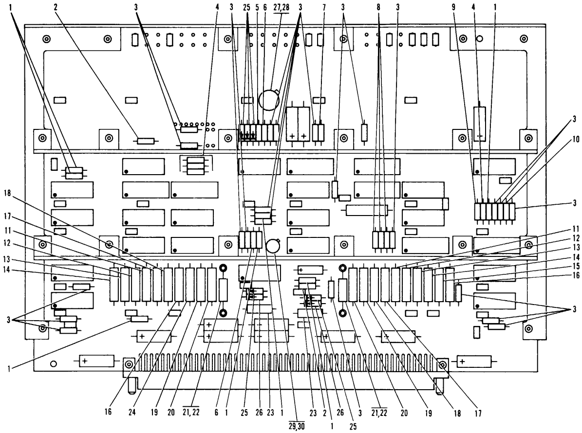
Figure 16. Type 6CCL Circuit Card Assembly (Sheet 1 of 2)
