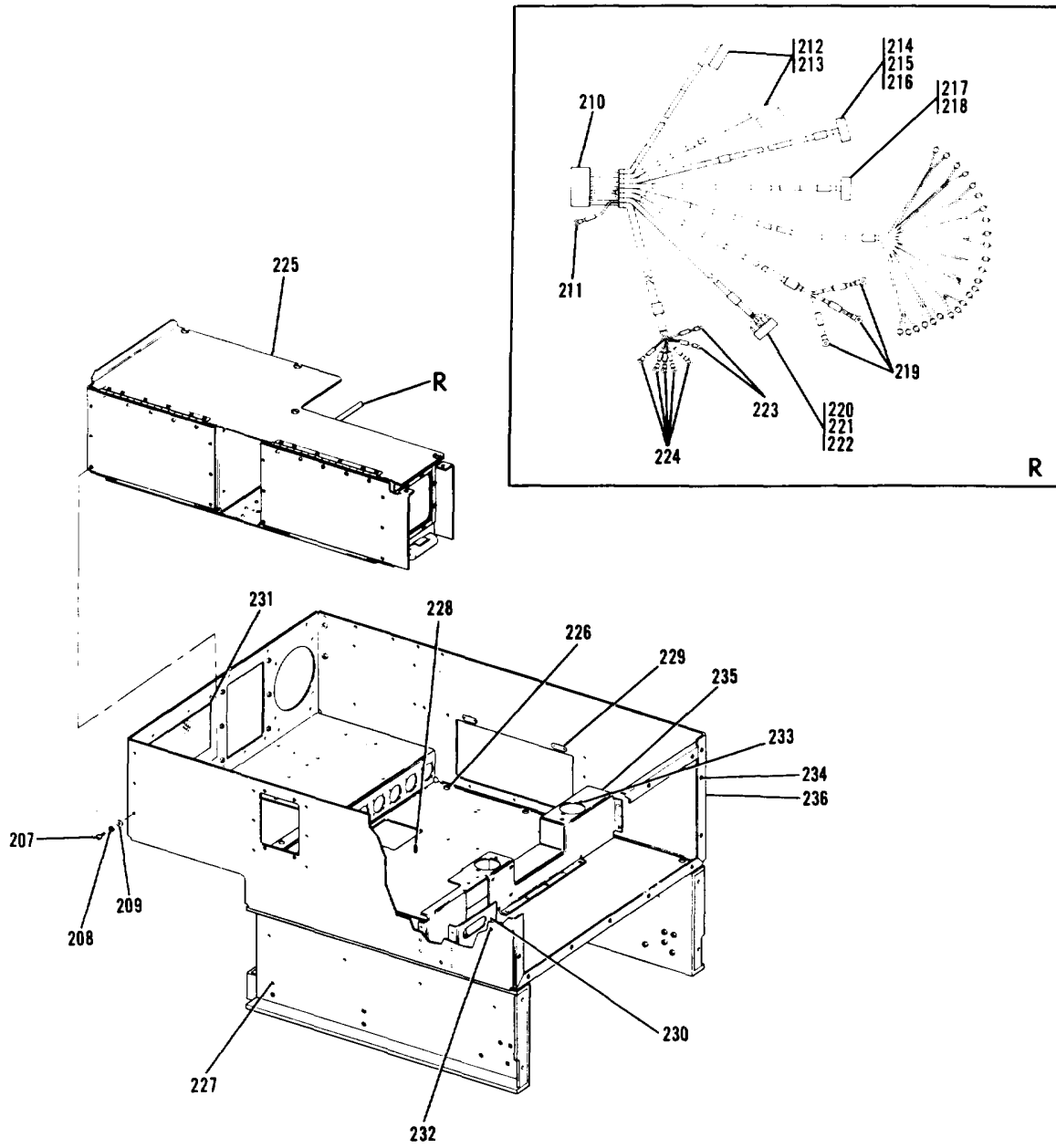
Figure 55. 3-Phase, 115V, 208V, 230V, 400 Hz Base Assembly (Sheet 4 of 4)
