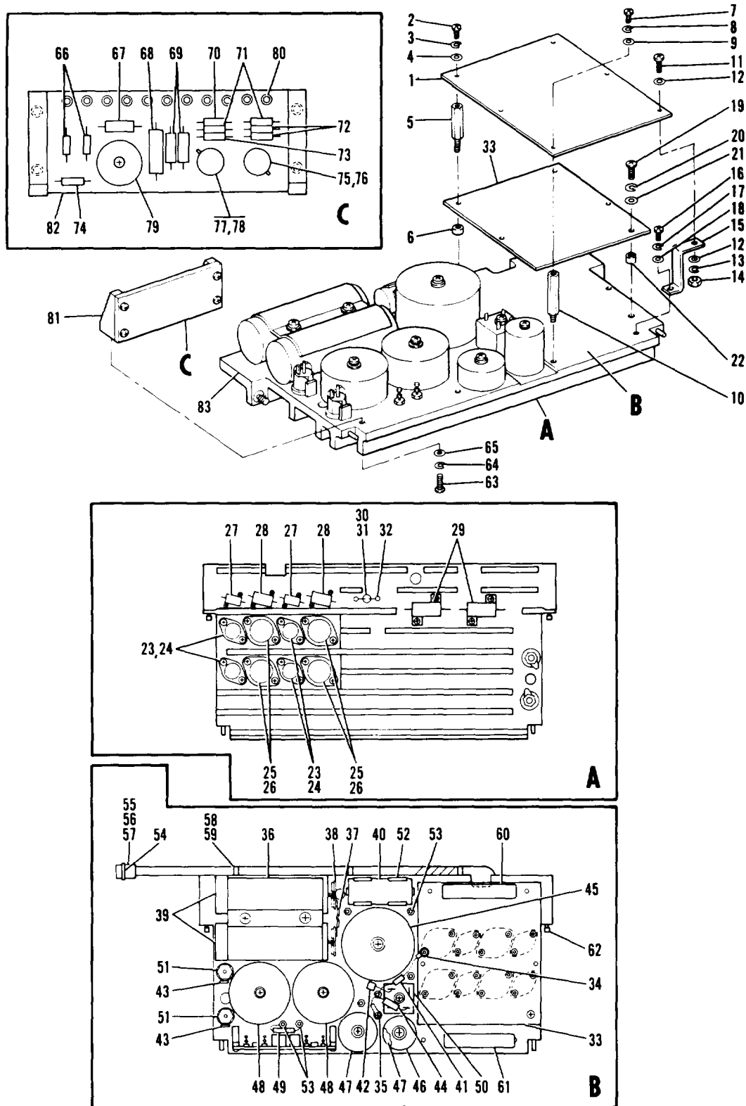
Figure 36. +40V Power Supply Assembly
