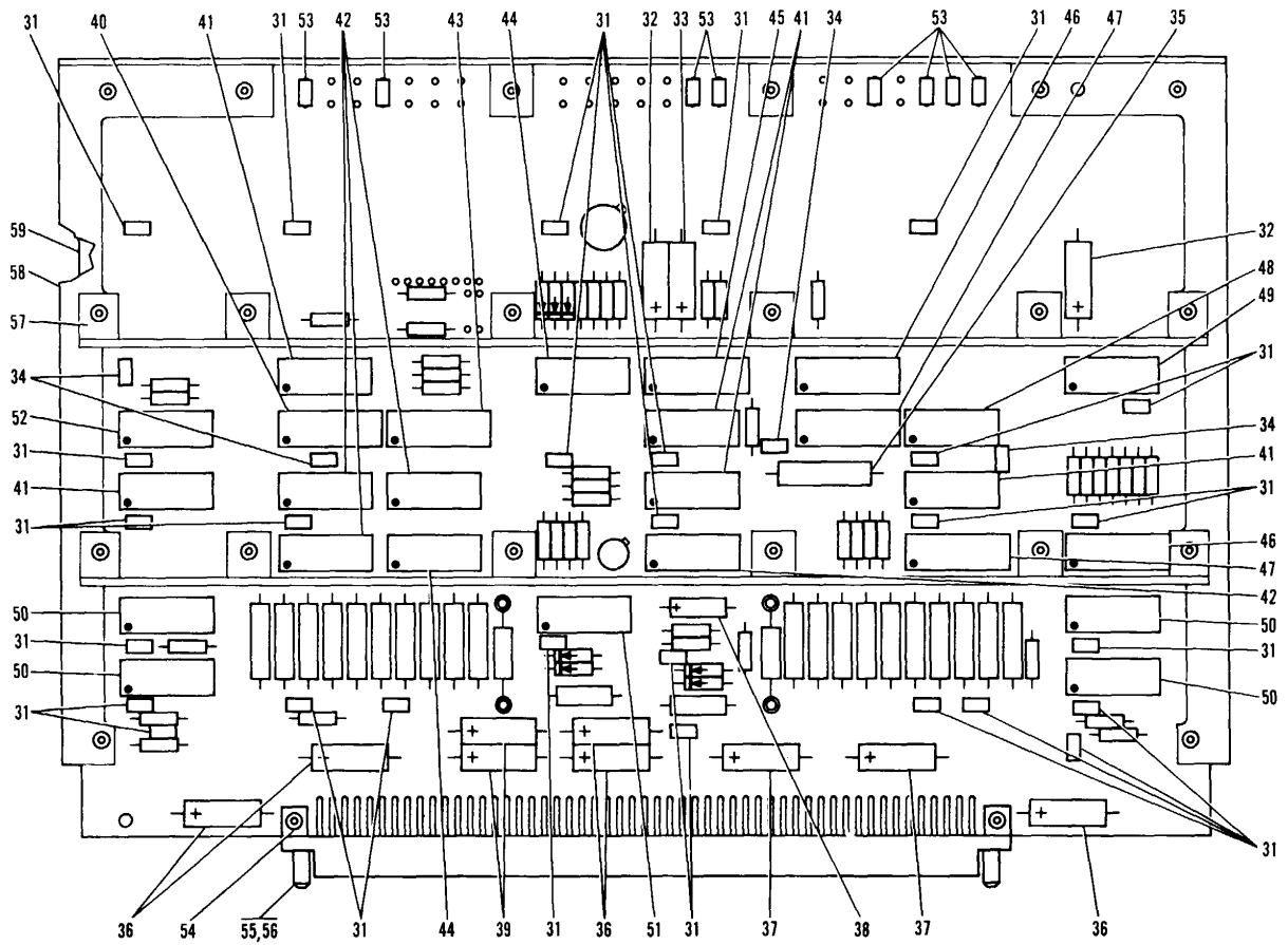
Figure 16. Type 6CCL Circuit Card Assembly (Sheet 2 of 2)
