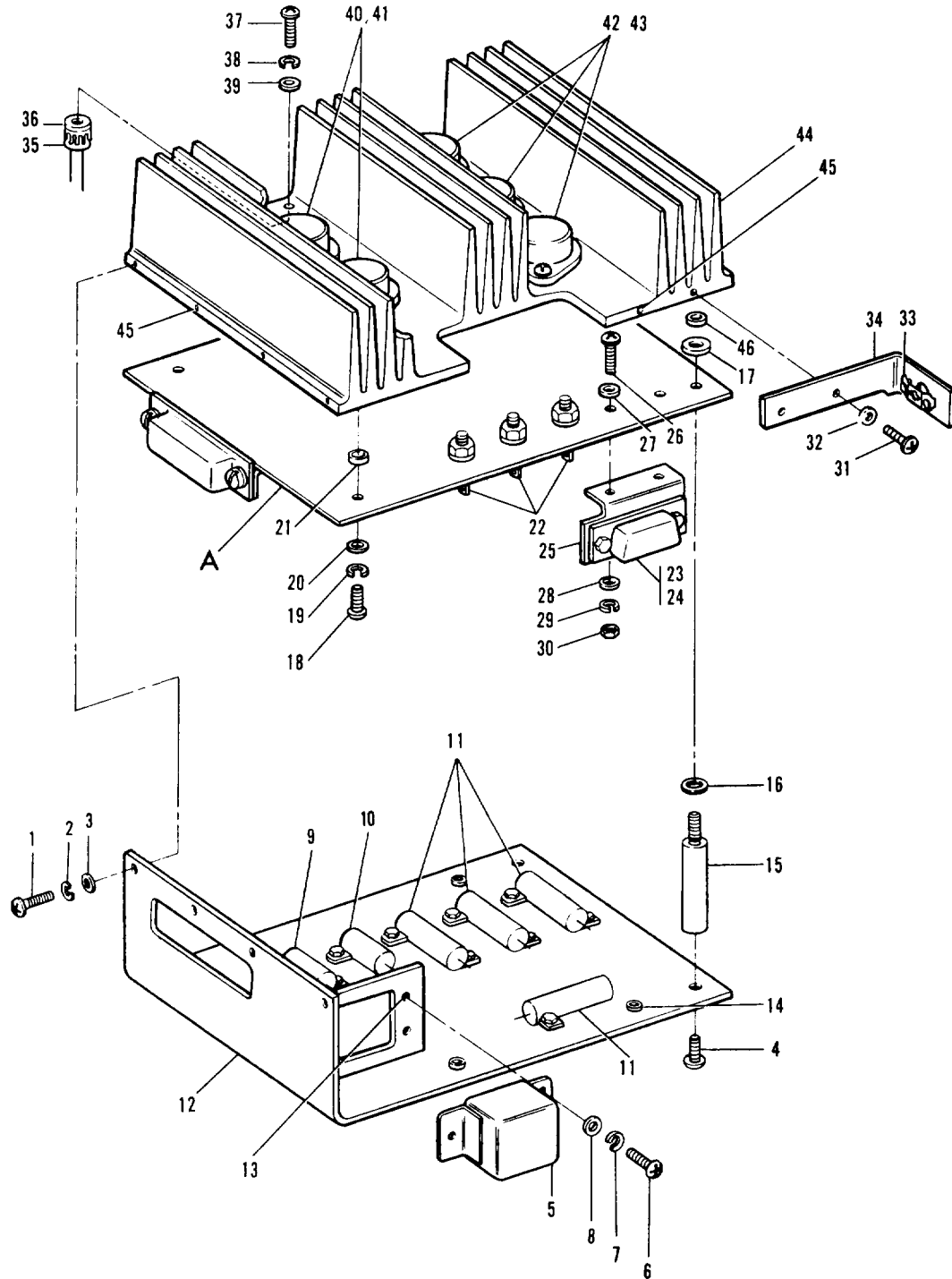
Figure 20. Power Amplifier Assembly (Sheet 1 of 2)
