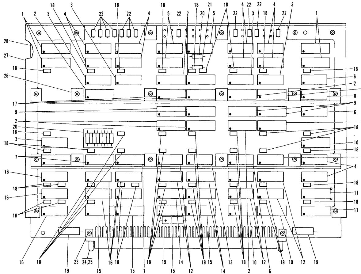
Figure 5. Type 6AEL Circuit Card Assembly
