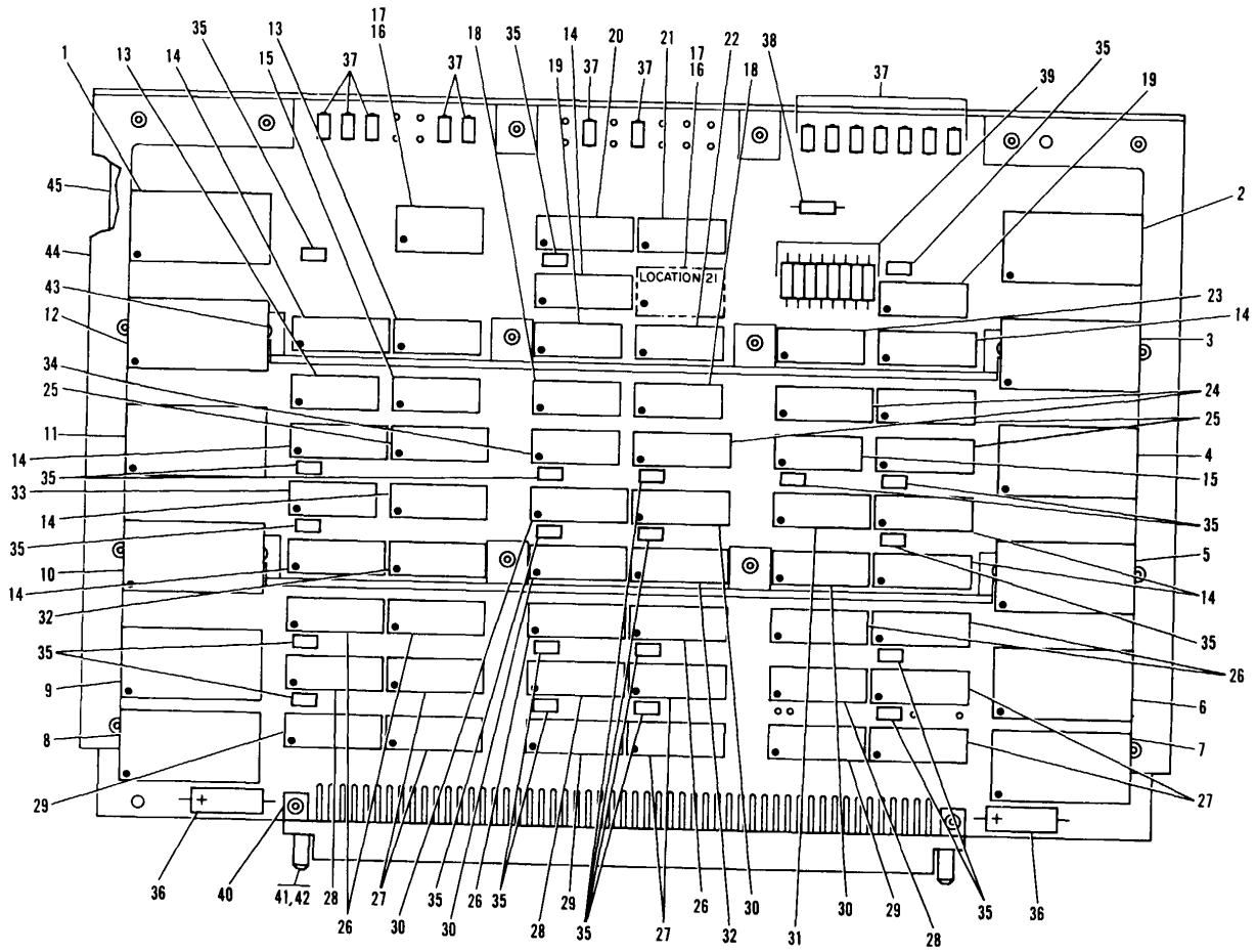
Figure 3. Type 9ACL Circuit Card Assembly
