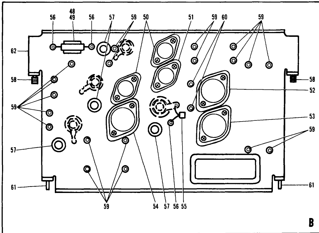
Figure 46. 5V, ± 11V, ± 15V Power Supply Assembly (Sheet 2 of 2)
