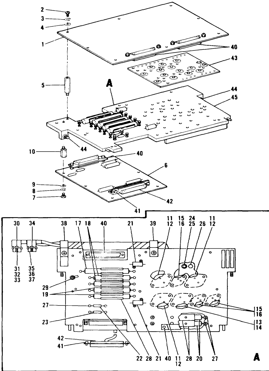
Figure 48. Auxiliary Temperature and Control Module
