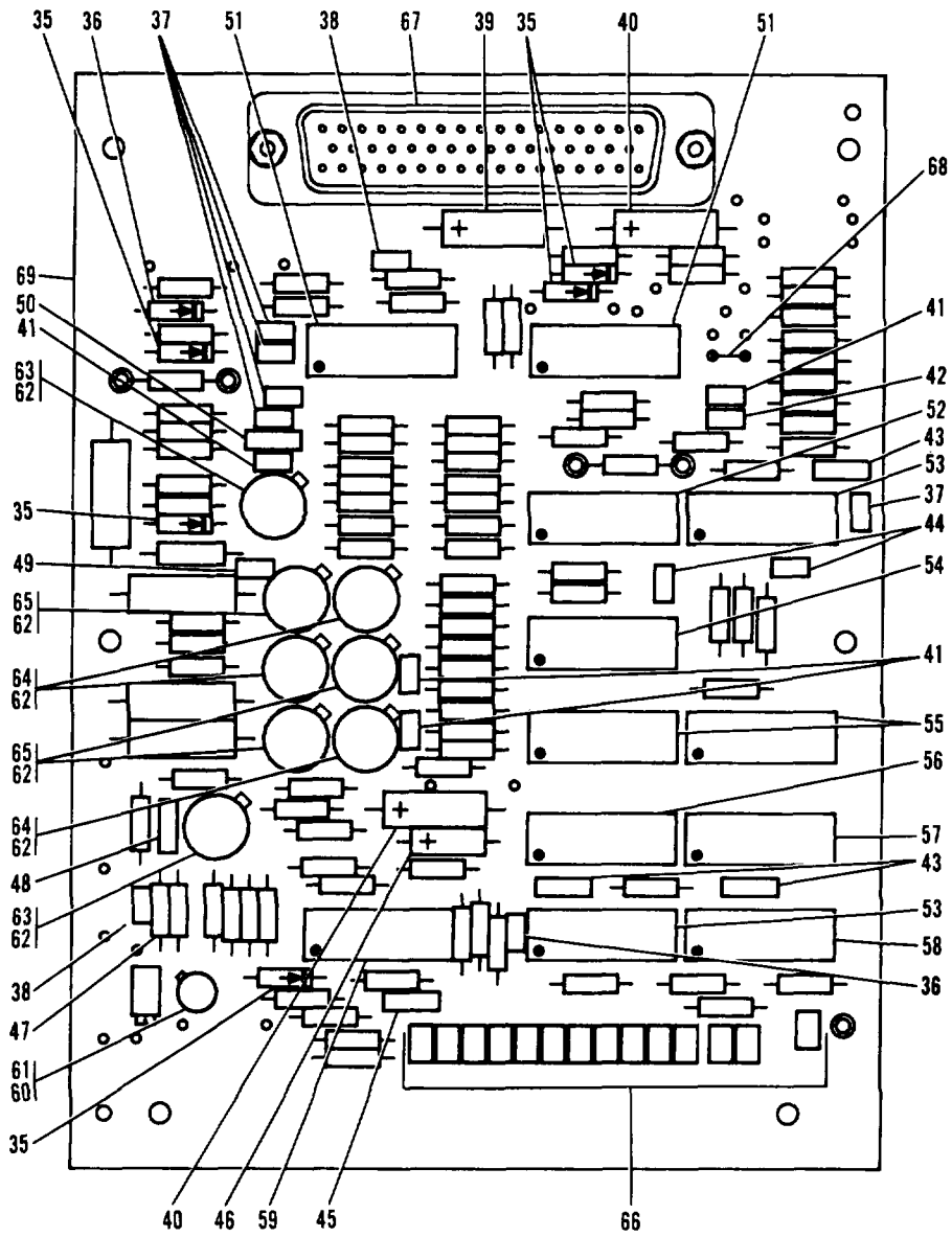
Figure 333-Phase Inverter Circuit Card subassembly (Sheet 2 of 3)
