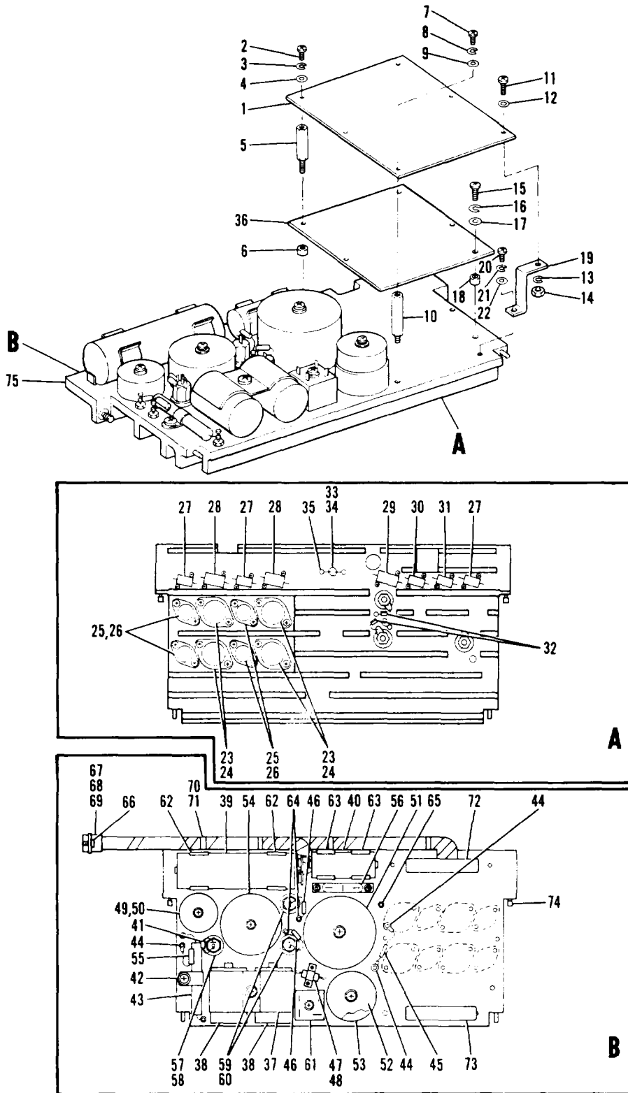
Figure 39. +5V Power supply Assembly
