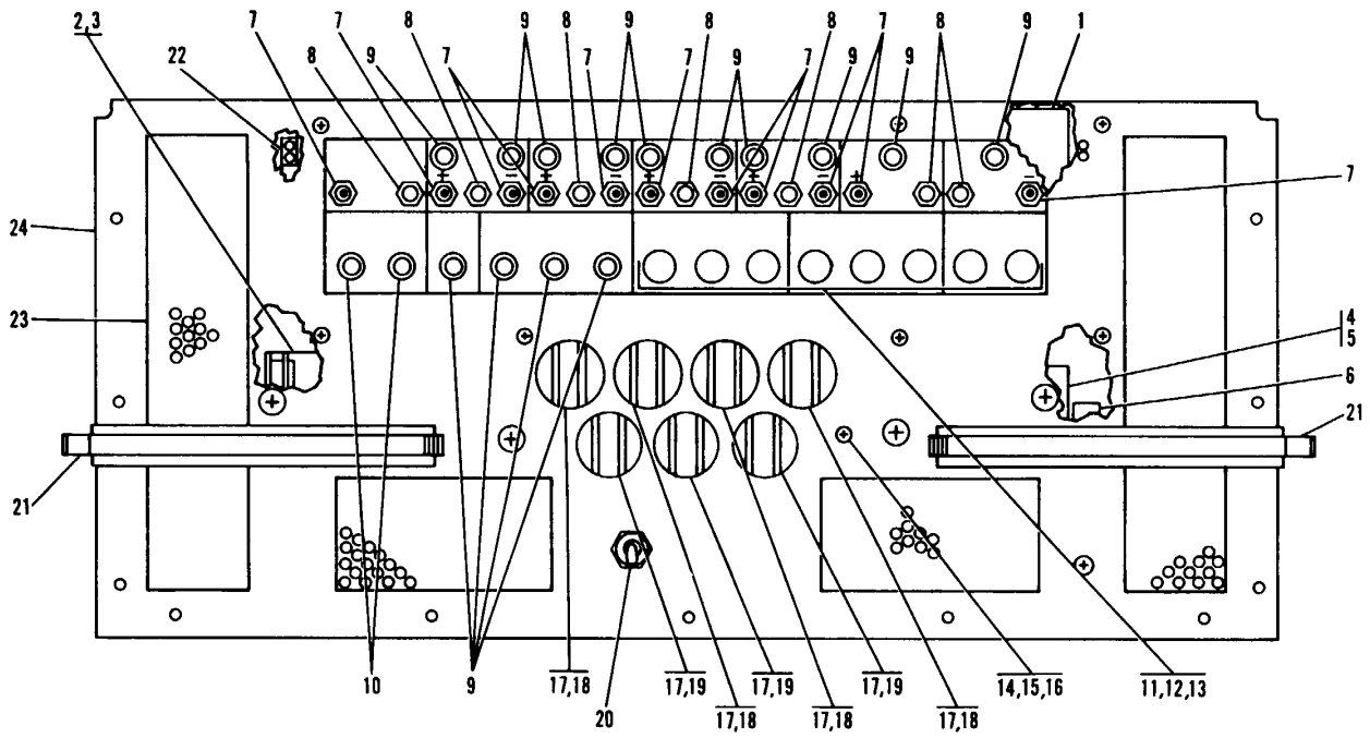
Figure 52. Power Supply Panel Assembly
