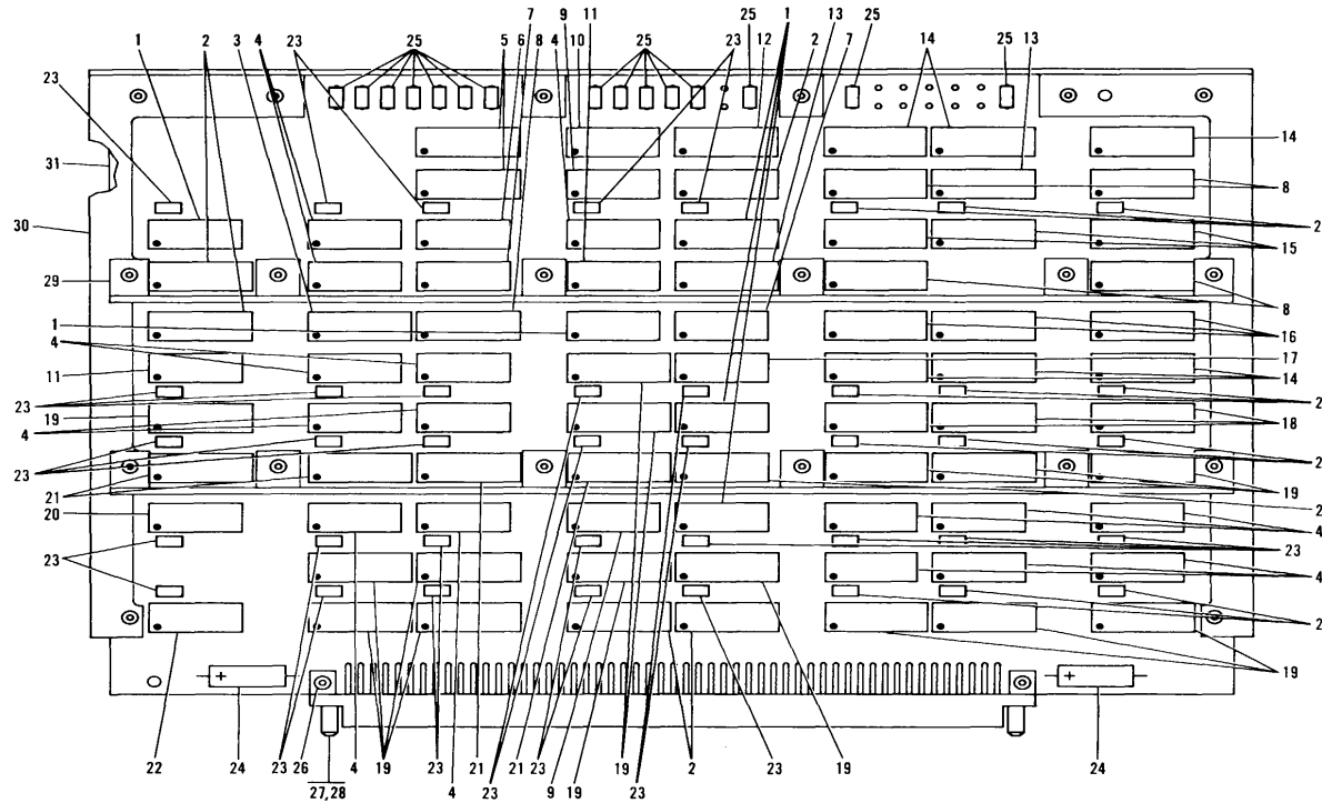
Figure 7. Type 6AGL Circuit Card Assembly
