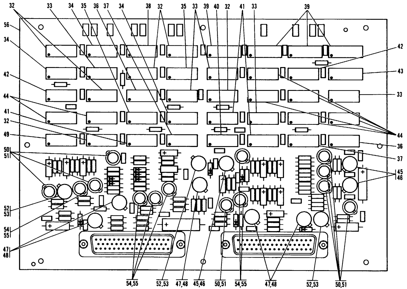
Figure 49. Power Control Circuit Card Subassembly (Sheet 3 of 3)
