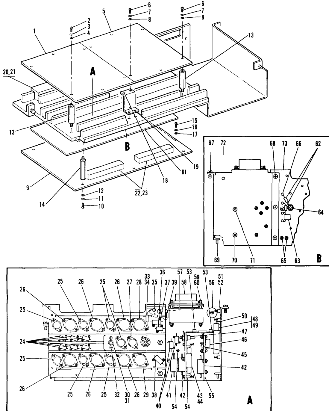
Figure 31. 3-Phase Inverter Speed Control and Preregulator Module
