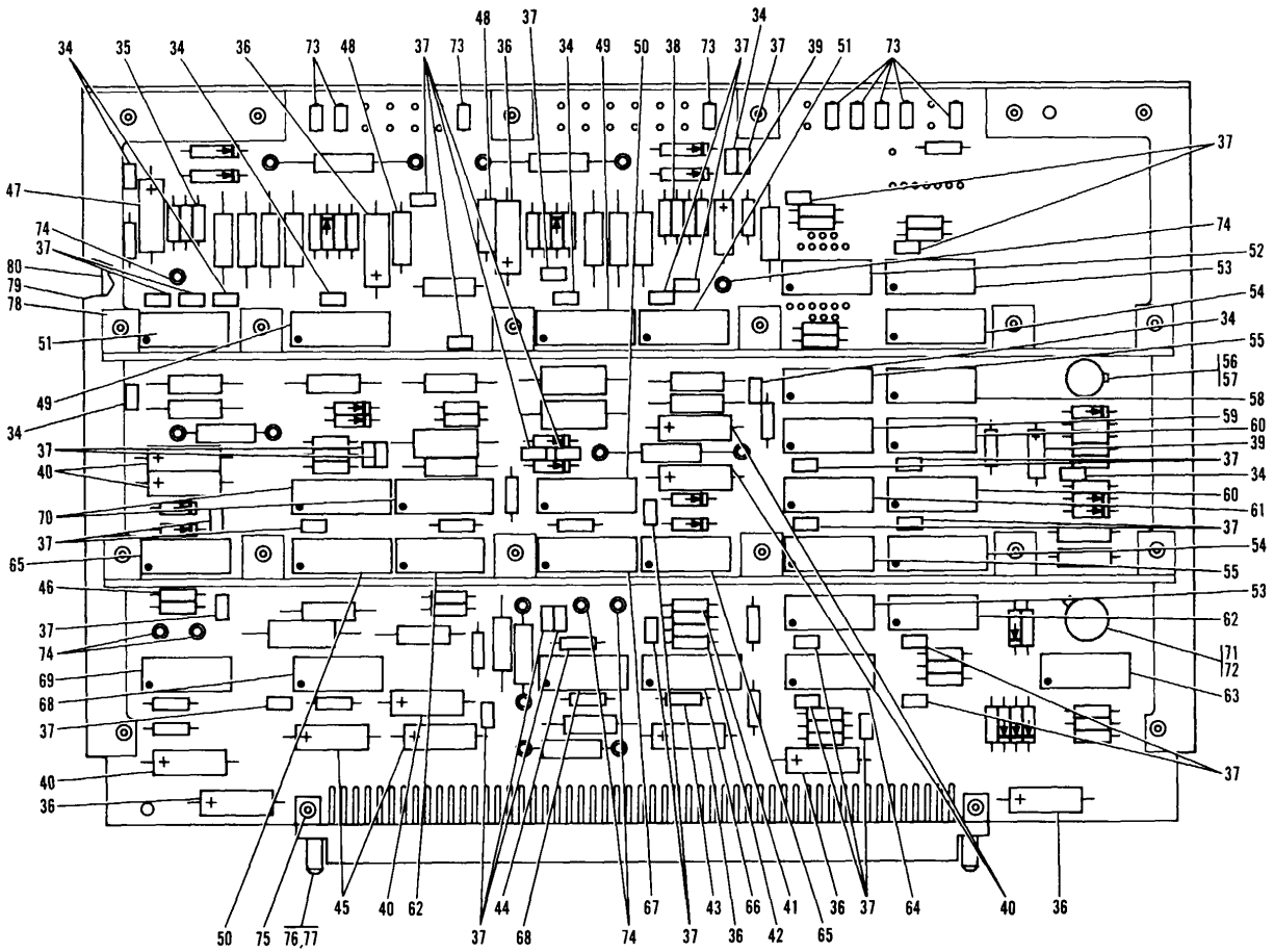
Figure 17. Type 6CBL Circuit Card Assembly (Sheet 2 of 2)
