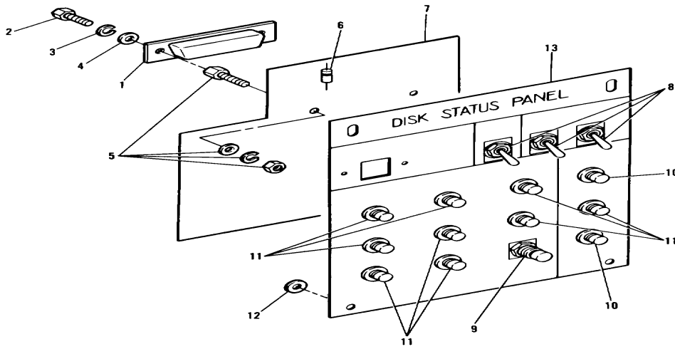
Figure 58. Status Panel Circuit Card Assembly
