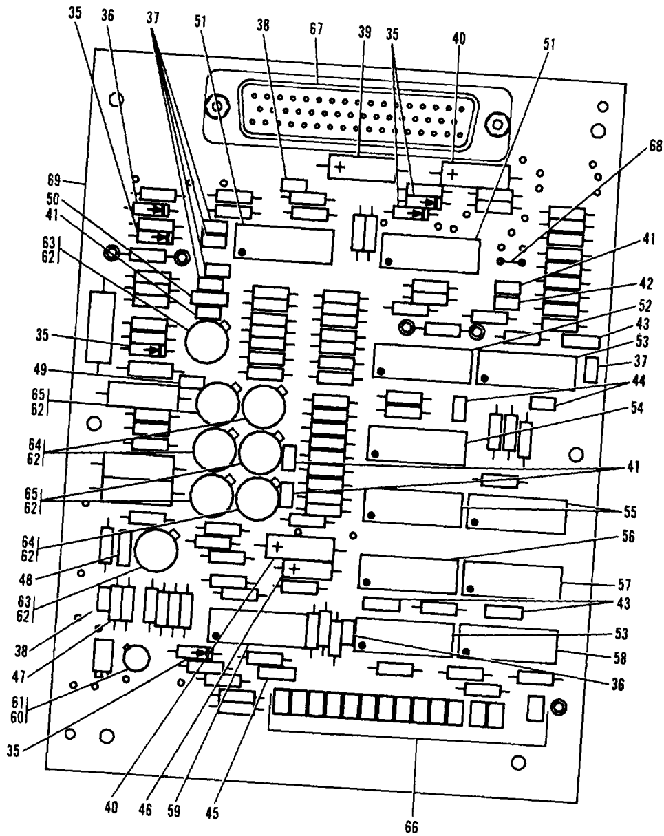
Figure 37-40V Inverter/Driver Circuit Card subassembly (Sheet 2 of 2)
