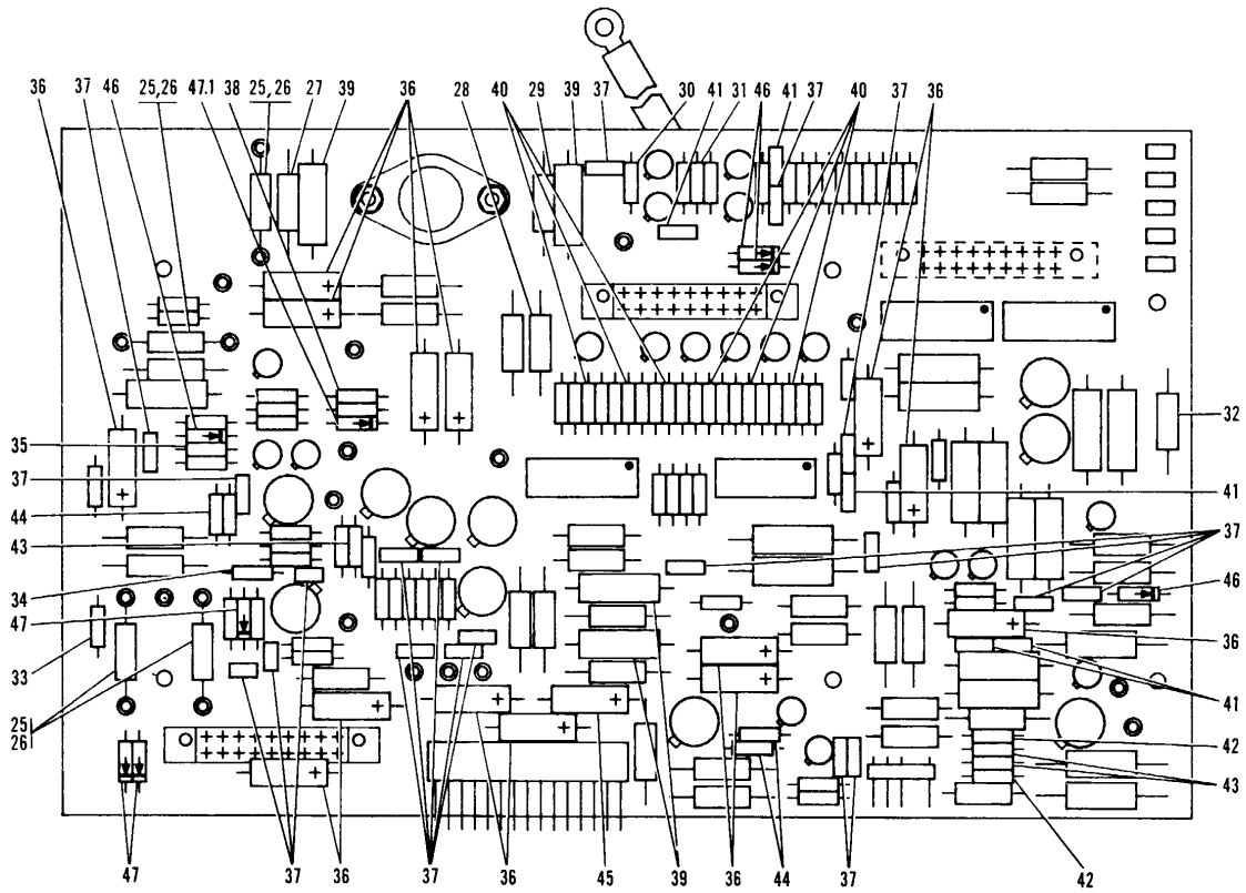
Figure 19. Head Select and Read Amplifier Circuit Card Assembly (Sheet 2 of 3)
