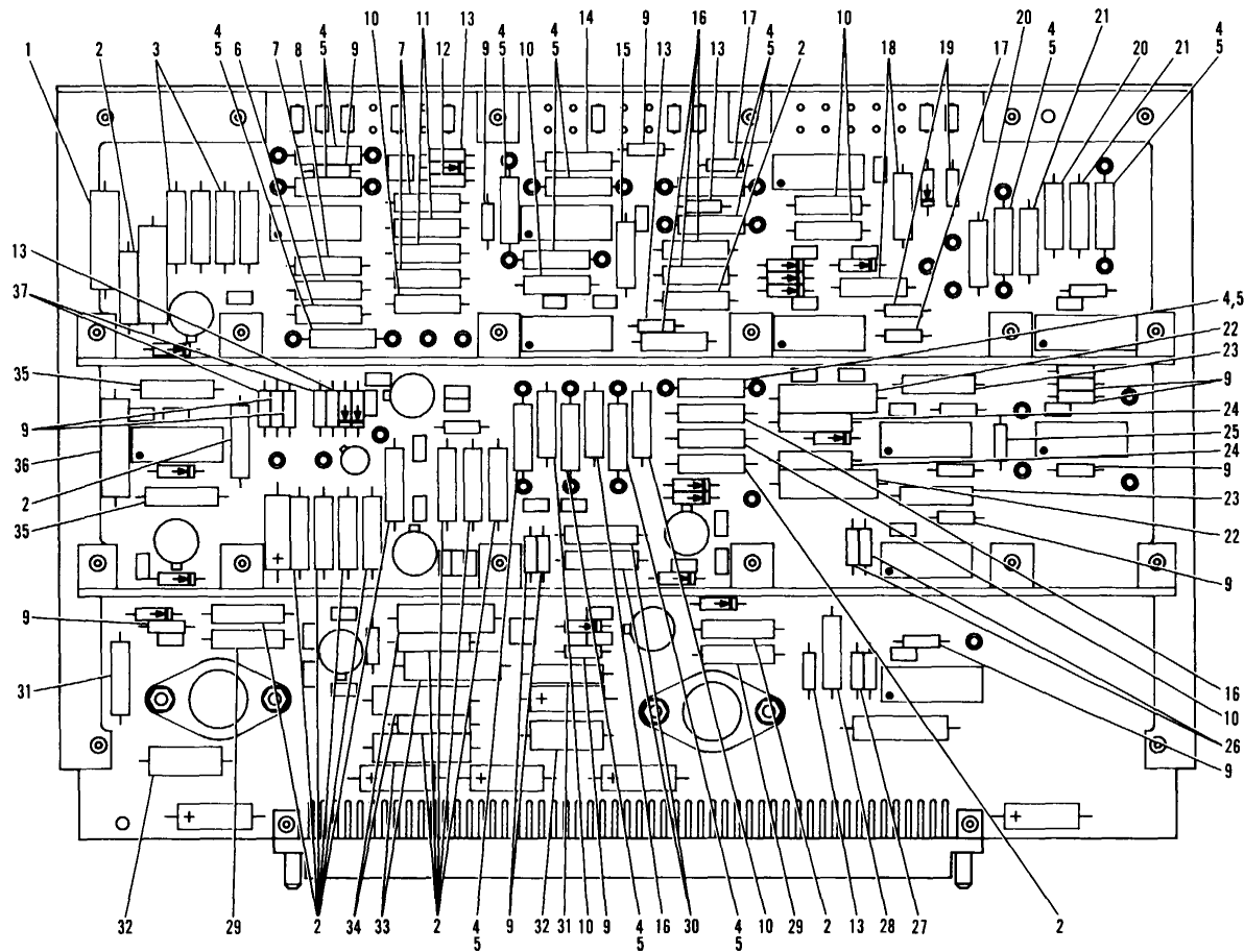
Figure 12. Type 6CGL Circuit Card Assembly (Sheet 1 of 2)
