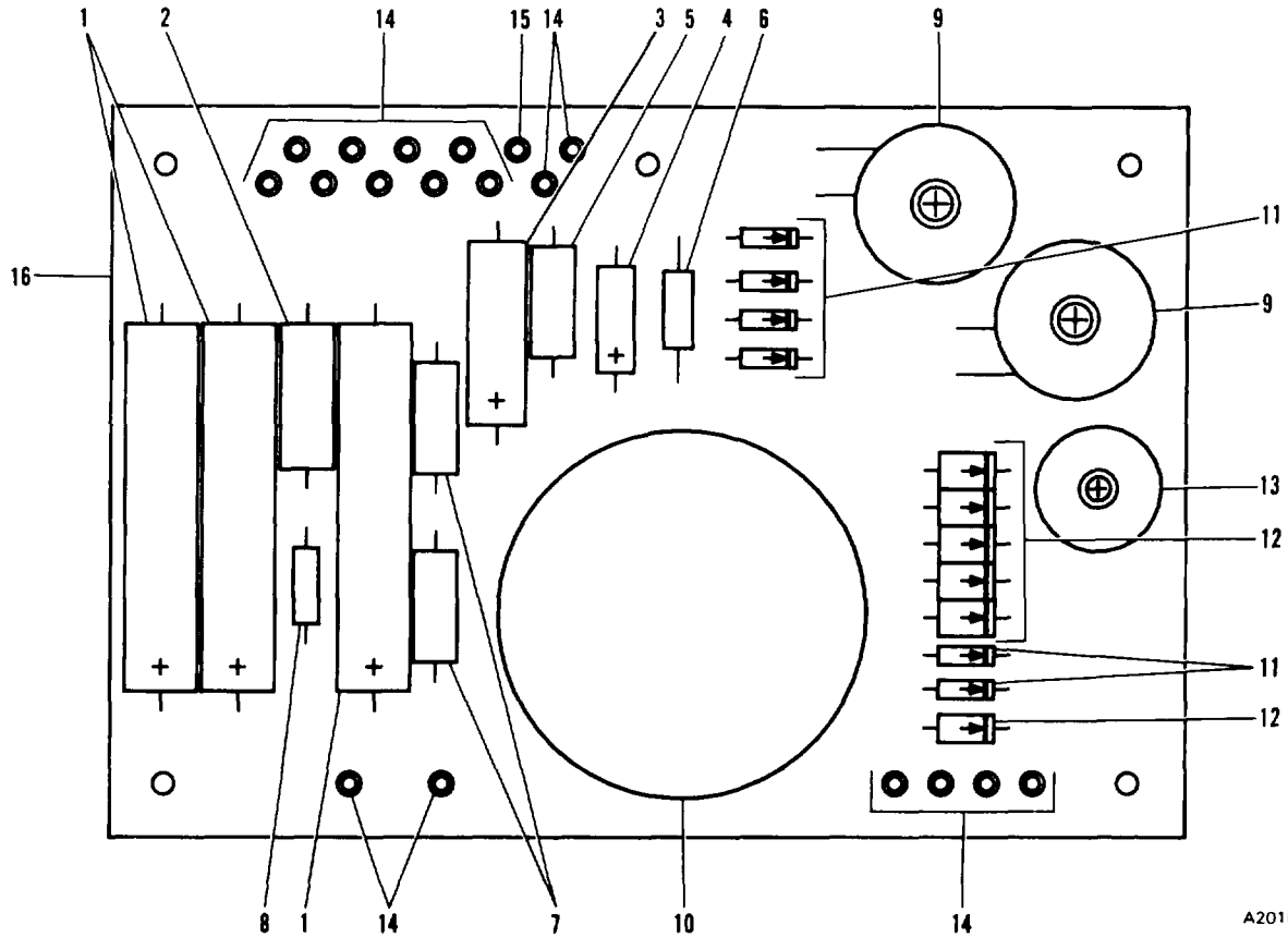
Figure 45. Disk Drive Output Circuit Card Subassembly
