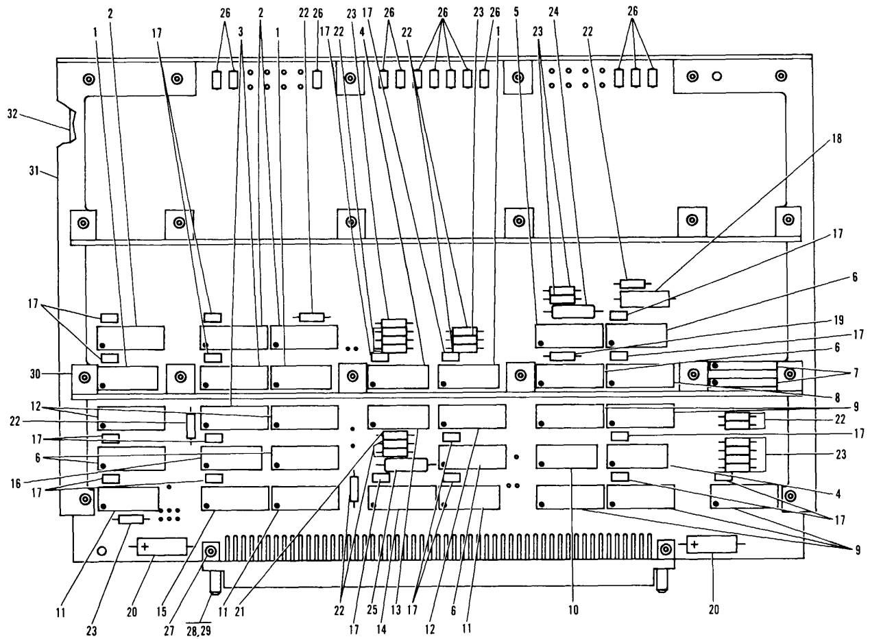
Figure 14. Type 6CEL Circuit Card Assembly
