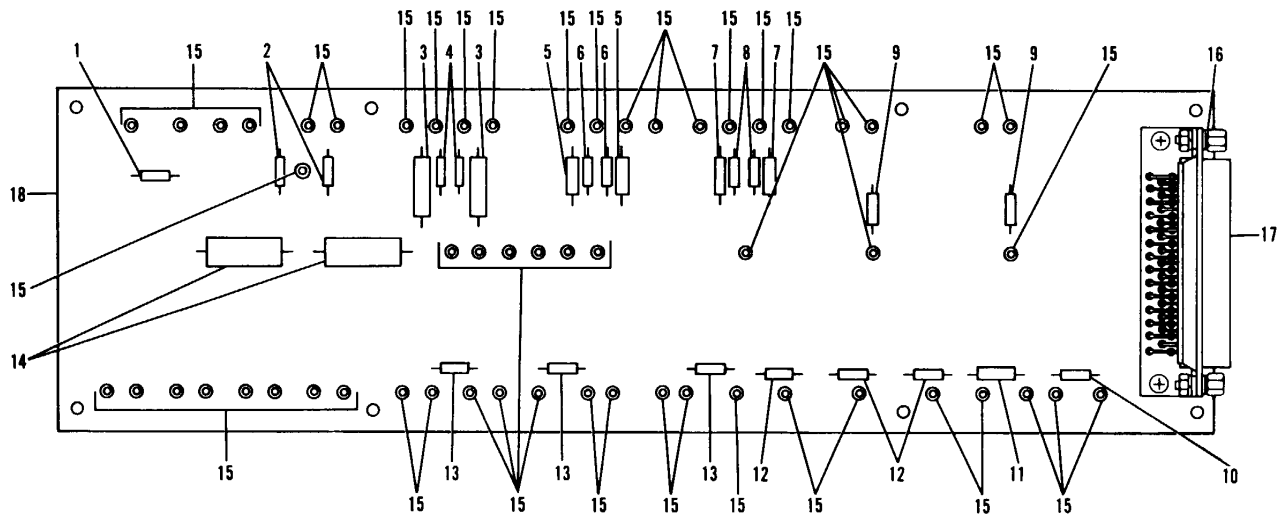
Figure 53. Power Supply Panel Circuit Card Subassembly
