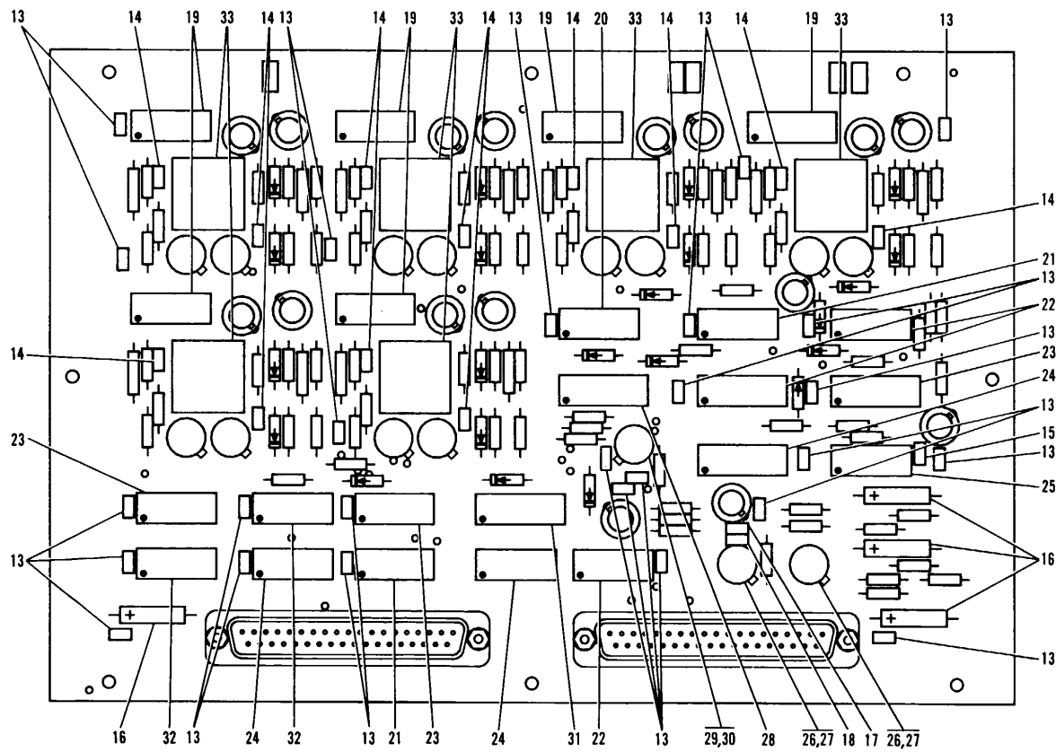
Figure 333-Phase Inverter Circuit Card subassembly (Sheet 3 of 3)
