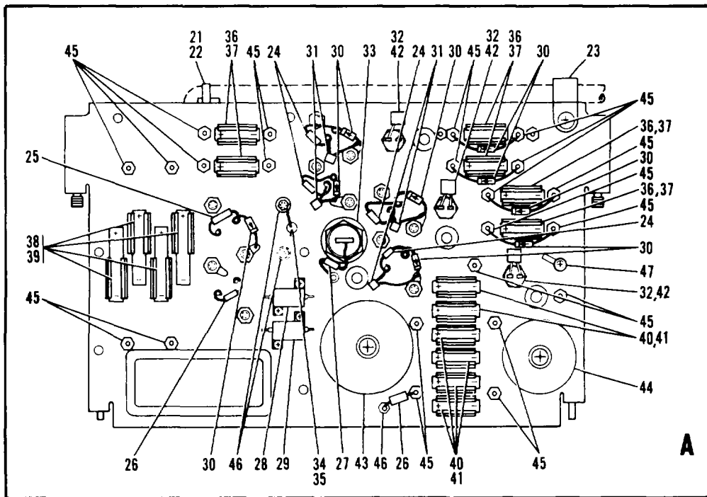
Figure 46. -5V, \pm 11V , \pm 15V Power Supply Assembly (Sheet 1 of 2)
