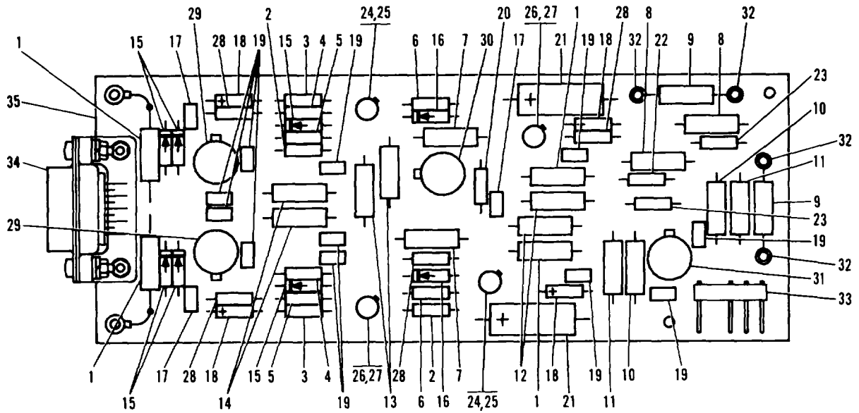
Figure 22. Servo Preamp Circuit Card Subassembly
