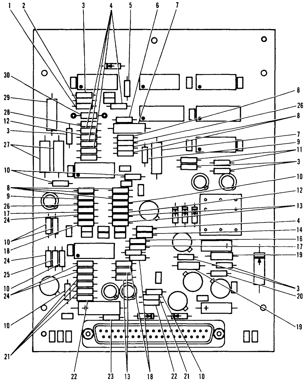
Figure 32. Preregulator Circuit Card Subassembly (Sheet 1 of 2)
