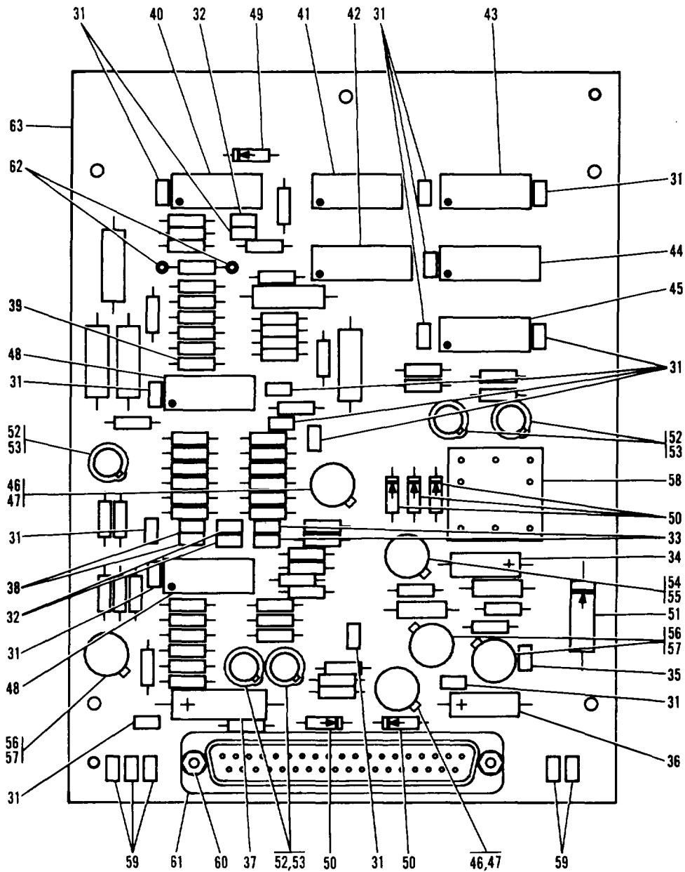
Figure 32. Preregulator Circuit Card Subassembly (Sheet 2 of 2)
