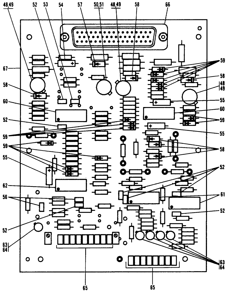
Figure 47. -5V, ± 11 V, ± 15V Regulator Circuit Card Subassembly (Sheet 2 of 2)
