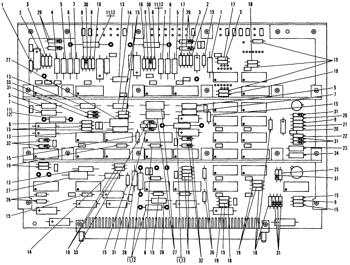
Figure 17. Type 6CBL Circuit Card Assembly (Sheet 1 of 2)
