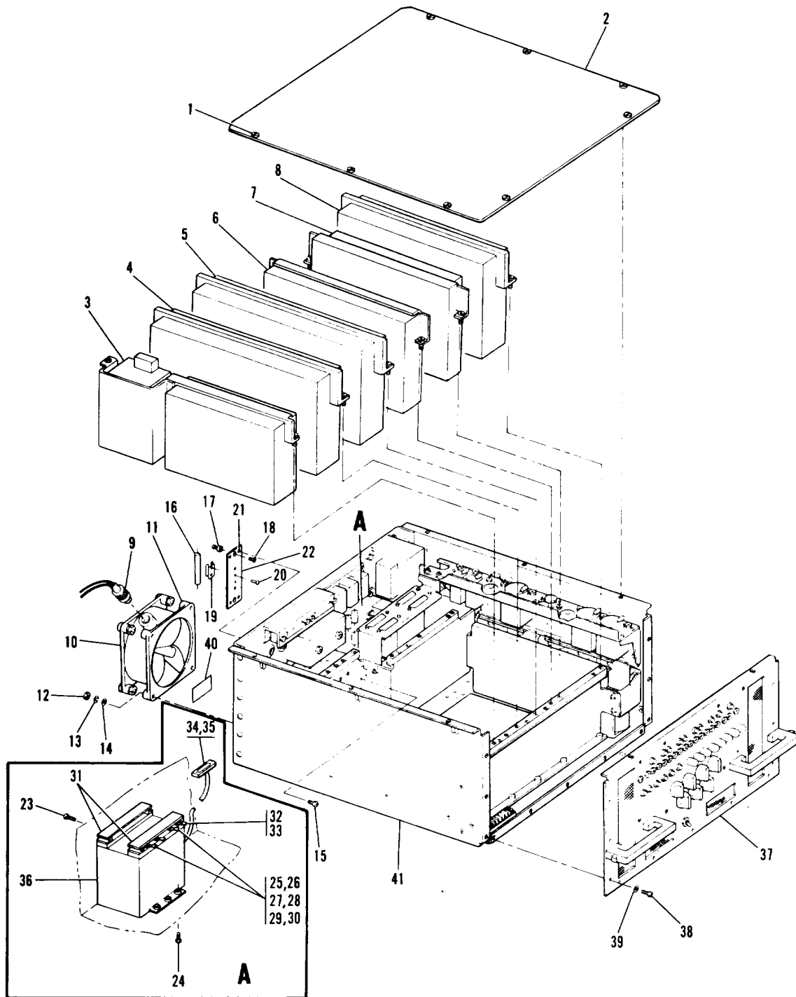
Figure 30. 3-Phase, 208V, 400 Hz Power Supply Assembly
