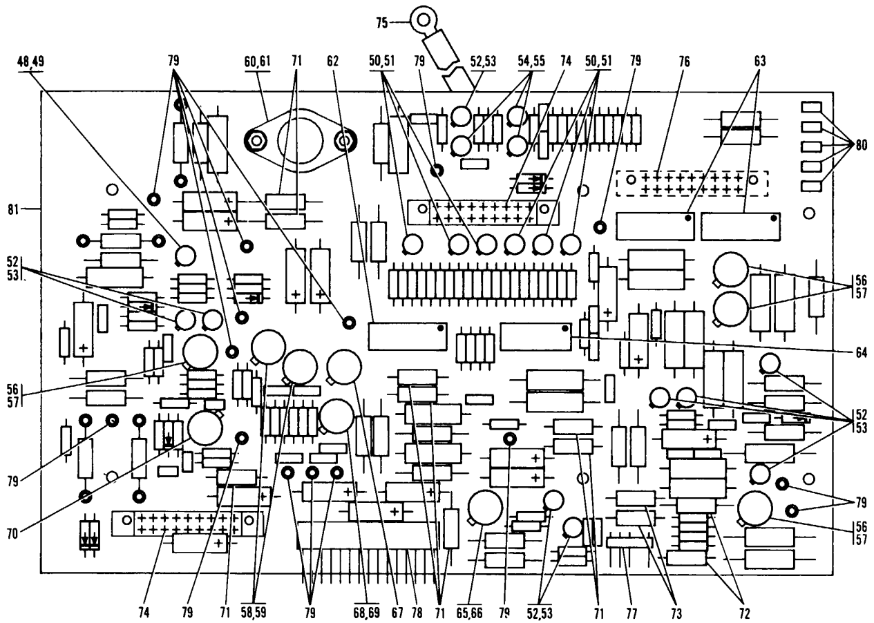
Figure 19. Head Select and Read Amplifier Circuit Card Assembly (Sheet 3 of 3)
