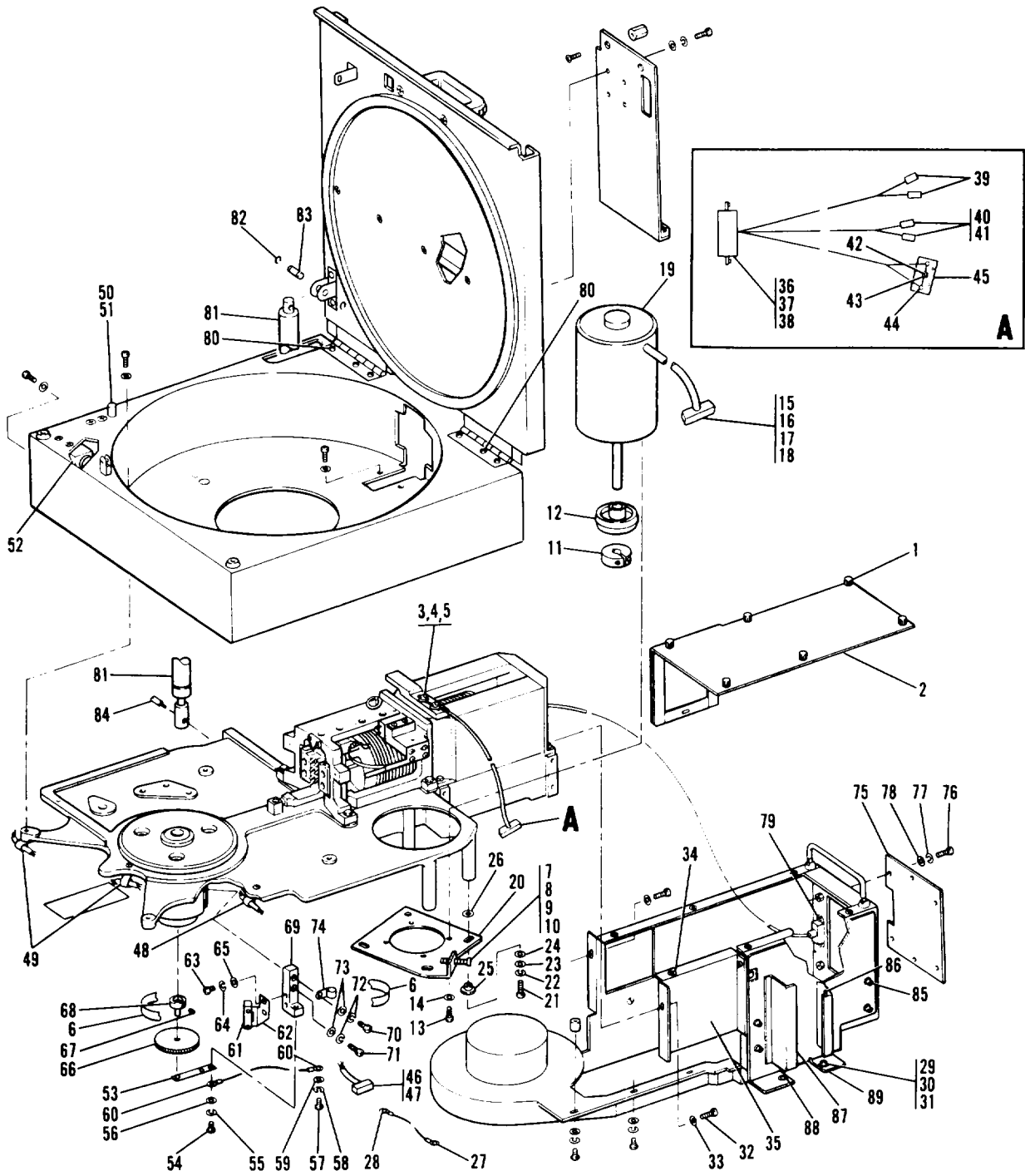
Figure 23. 80-Megabyte Deck Assembly (Sheet 1 of 2)
