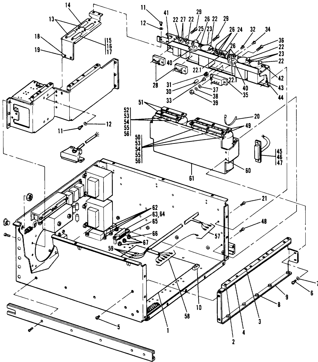
Figure 54. Power Supply Enclosure Assembly (Sheet 1 of 2)
