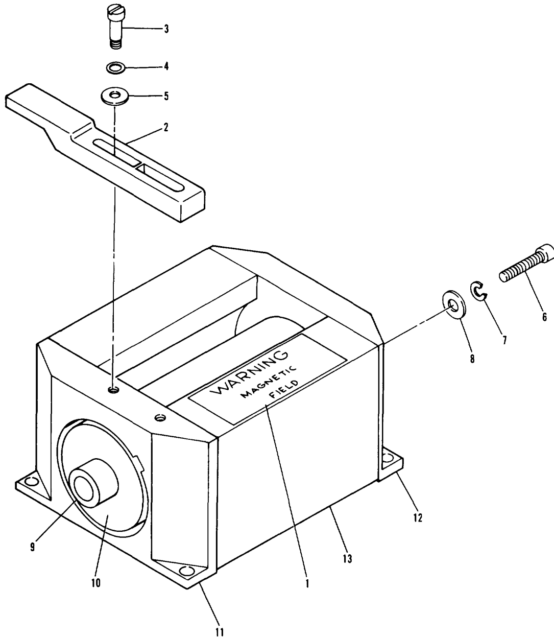
Figure 27. Magnet Assembly
