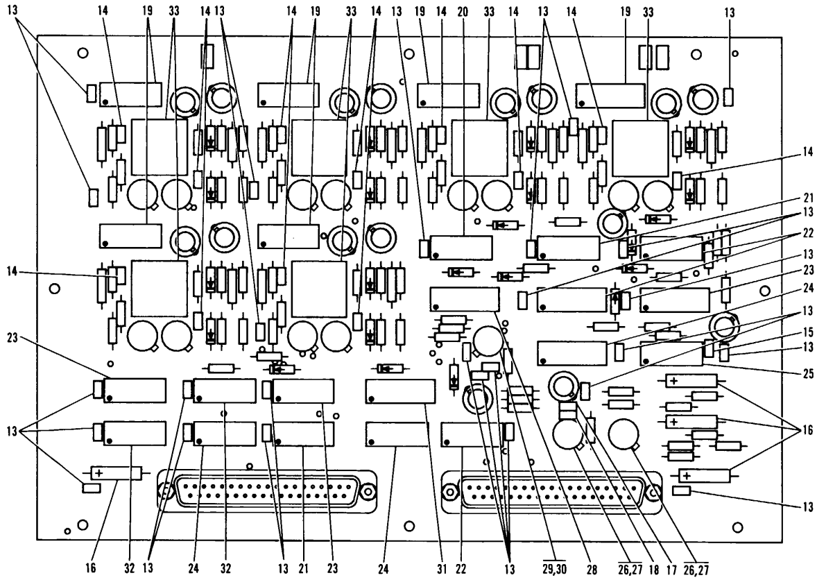
Figure 34. speed Control Circuit Card subassembly (Sheet 1 of 2)
