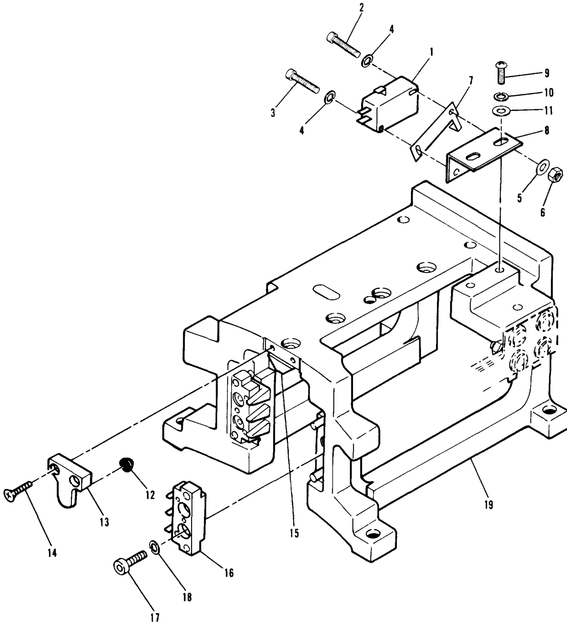
Figure 26. Rail Bracket Assembly
