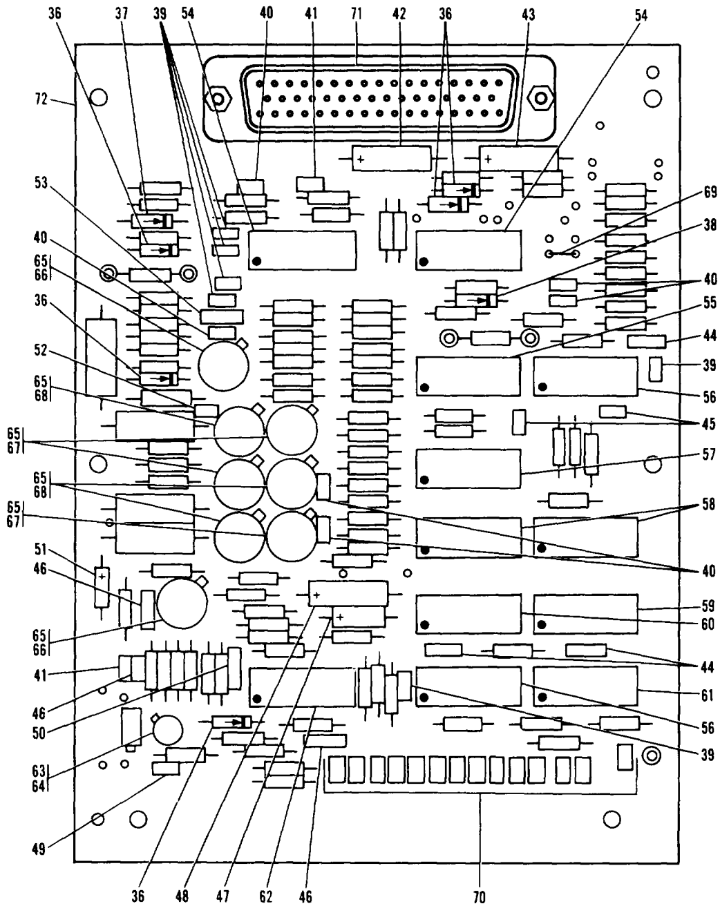
Figure 43 Disk Drive Inverter/Driver Circuit Card Subassembly (Sheet 2 of 2)
