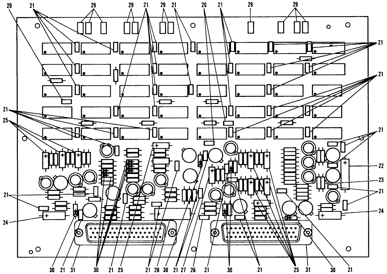
Figure 49. Power Control Circuit Card Subassembly (Sheet 2 of 3)
