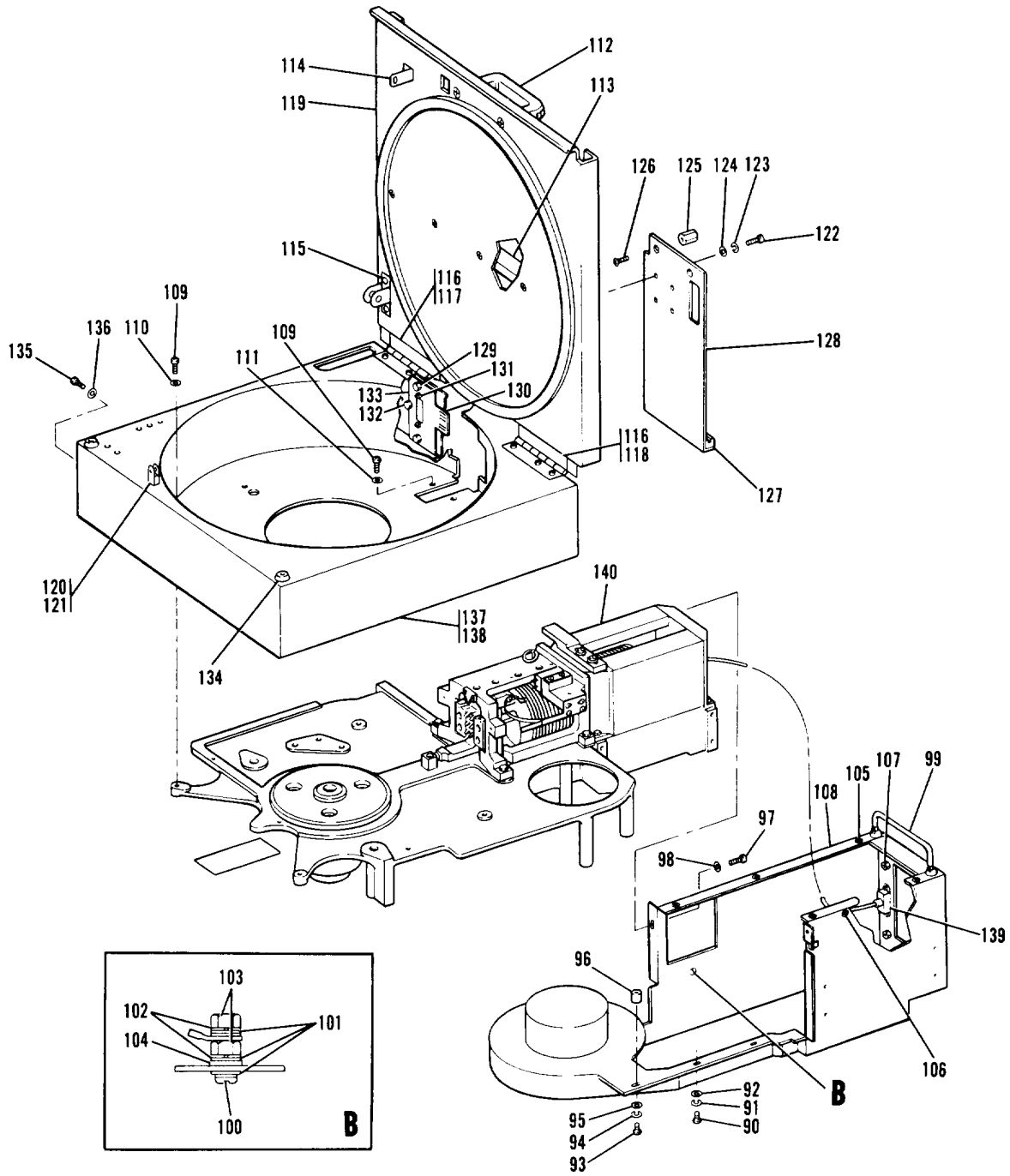
Figure 23. 80-Megabyte Deck Assembly (Sheet 2 of 2)
