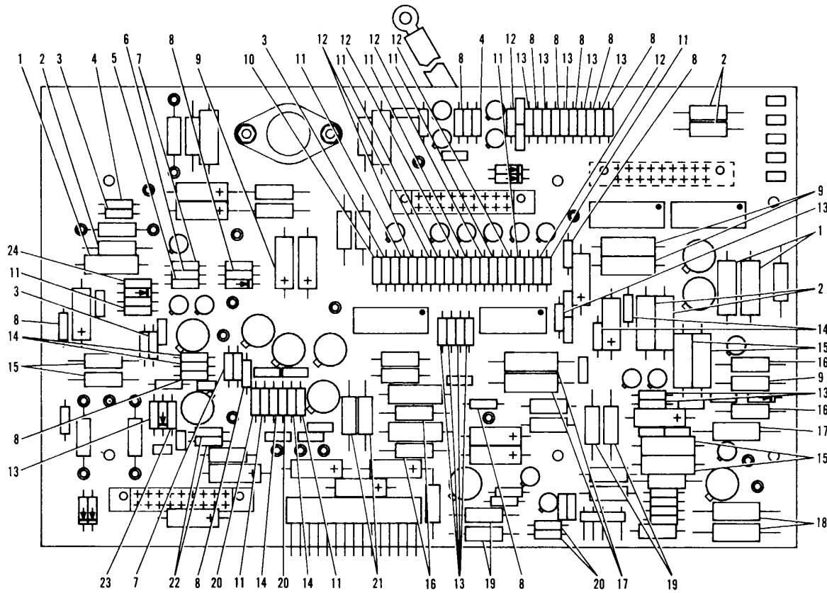
Figure 19. Head Select and Read Amplifier Circuit Card Assembly (Sheet 1 of 3)
