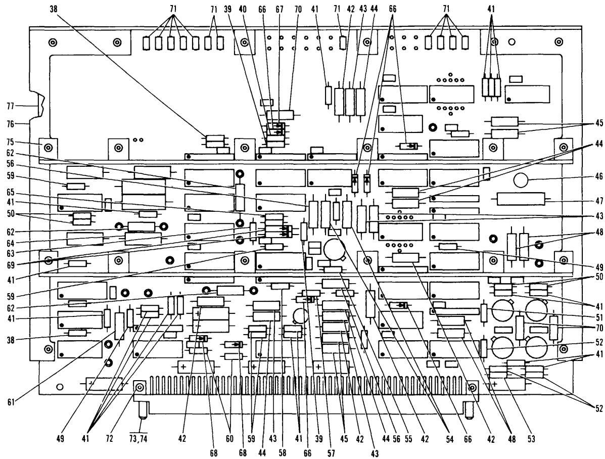
Figure 10. Type 6DAL Circuit Card Assembly (Sheet 2 of 2)
