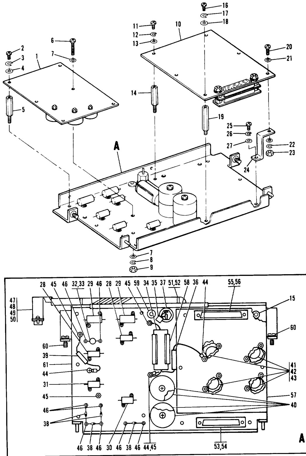
Figure 42. Disk Drive Power supply Module
