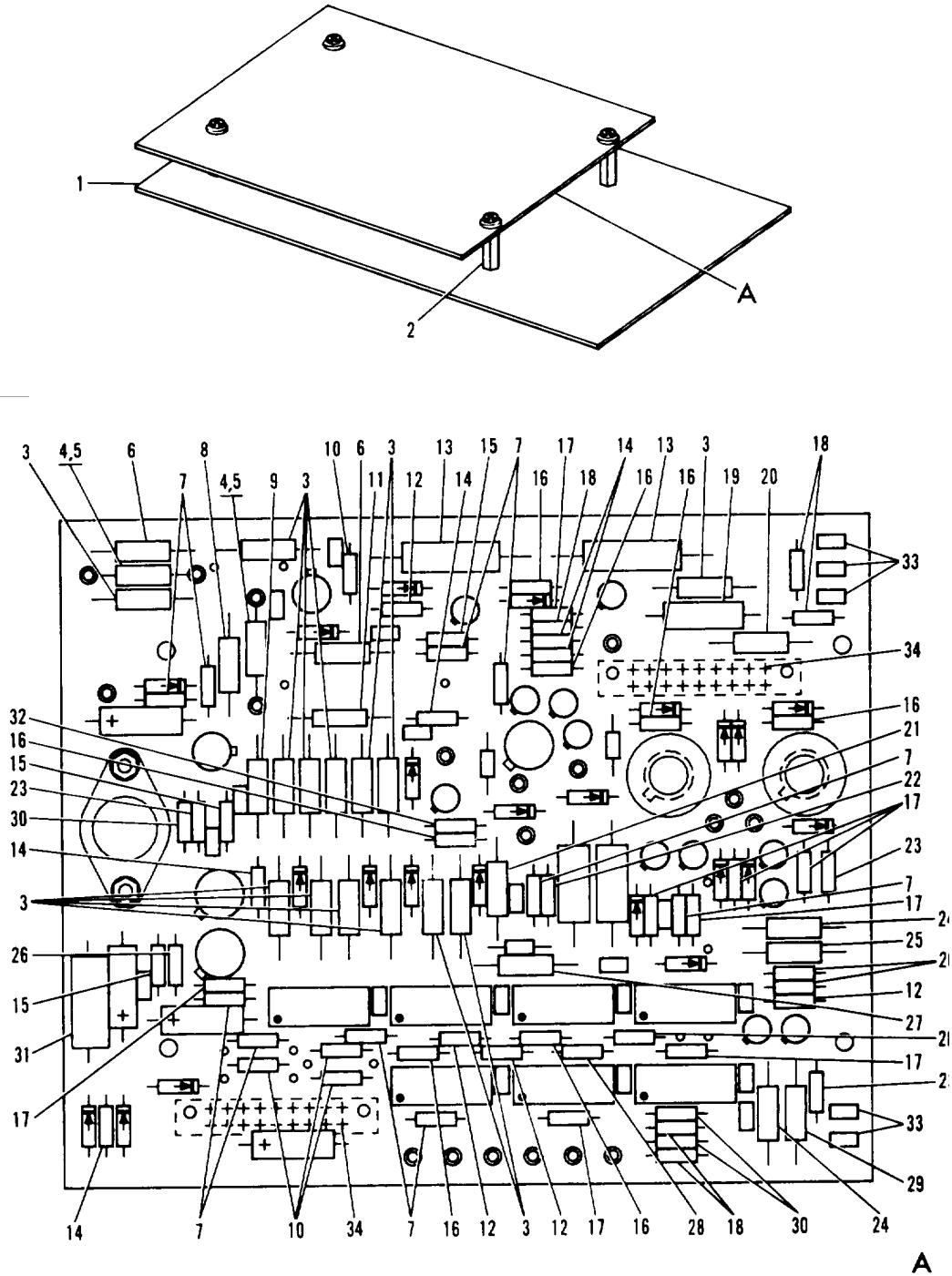
Figure 18. Read/Write Assembly (Sheet 1 of 2)
