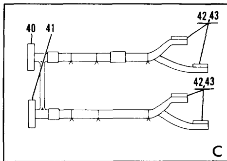
Figure 1. MU-695/TYQ Disk Memory Unit (Sheet 2 of 2)
