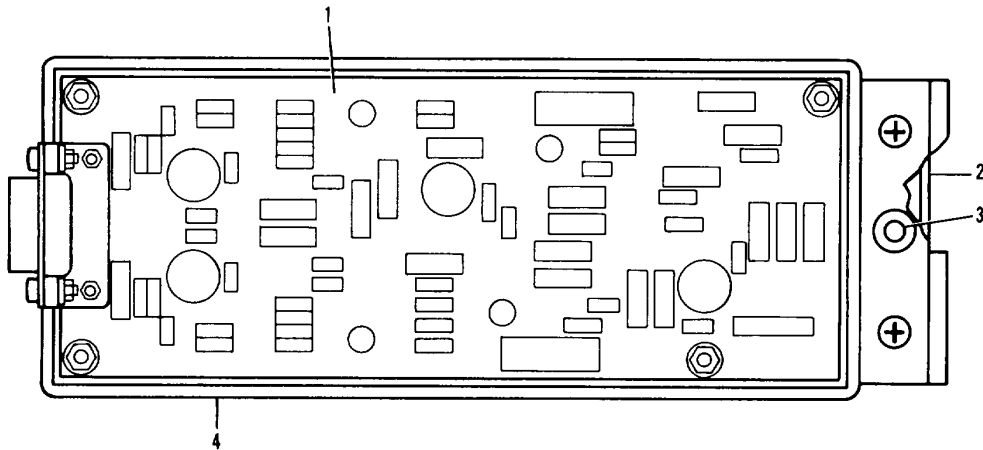
Figure 21. Servo Preamp Module
