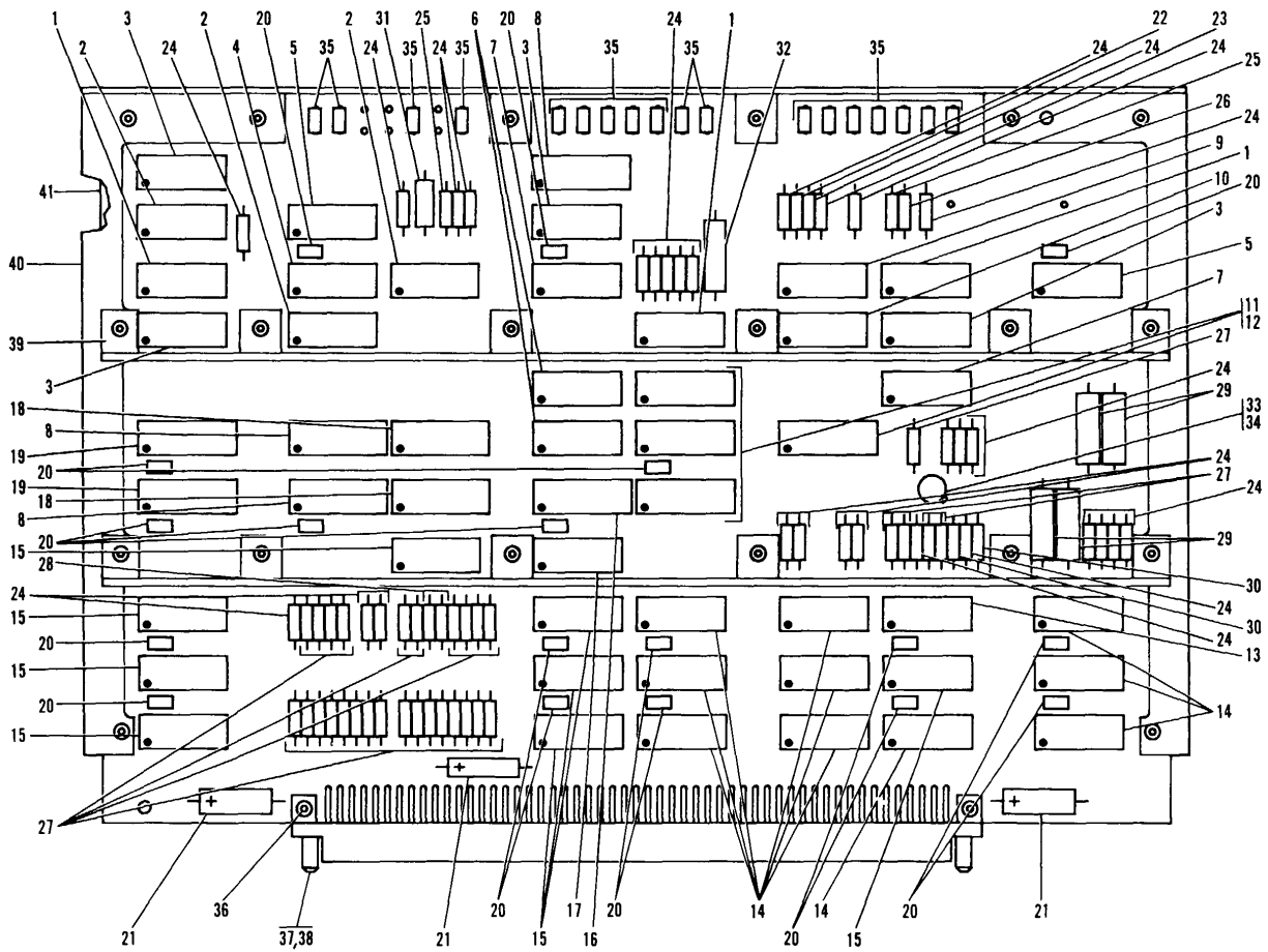
Figure 15. Type 6CDL Circuit Card Assembly
