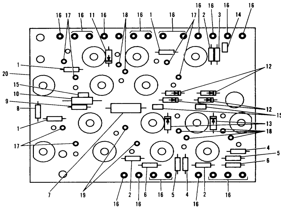
Figure 51. Power Control Transistor Interface Circuit Card Subassembly
