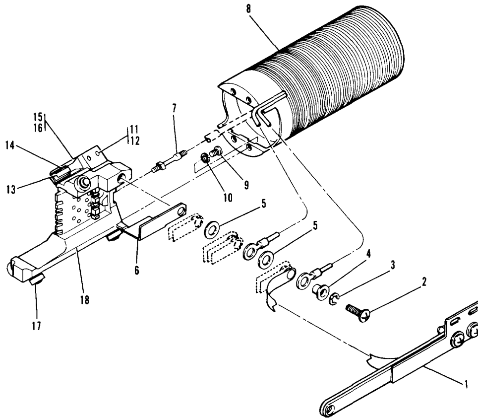
Figure 29. Carriage and Coil Assembly
