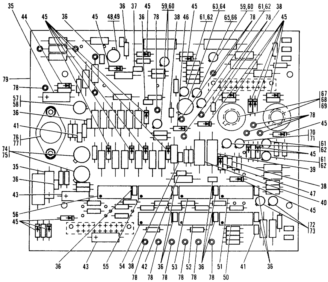
Figure 18. Read/Write Assembly (Sheet 2 of 2)
