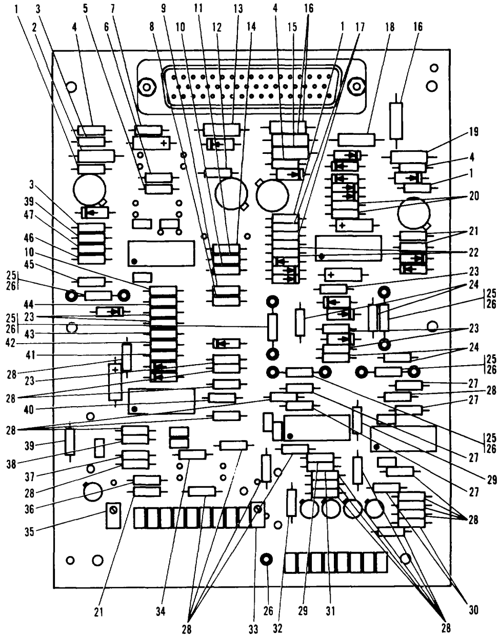
Figure 47. -5V, ±11V, ±15V Regulator Circuit Card Subassembly (Sheet 1 of 2)
