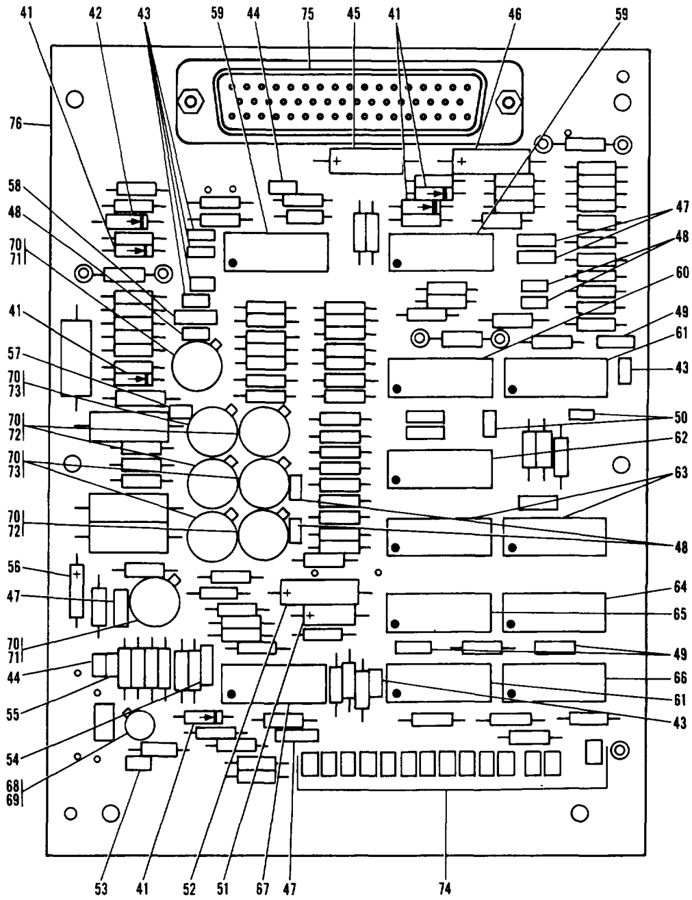
Figure 40+5V Inverter/Driver Circuit Card subassembly (Sheet 2 of 2)
