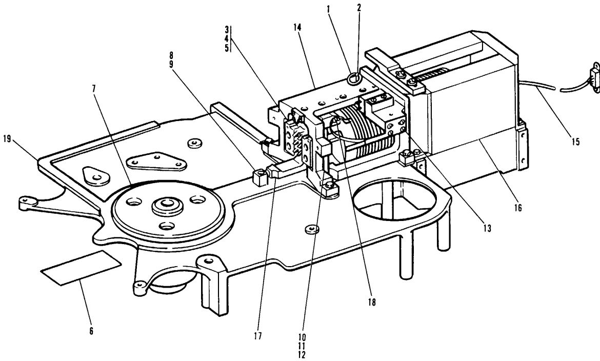
Figure 24. Disk Memory Drive Assembly
