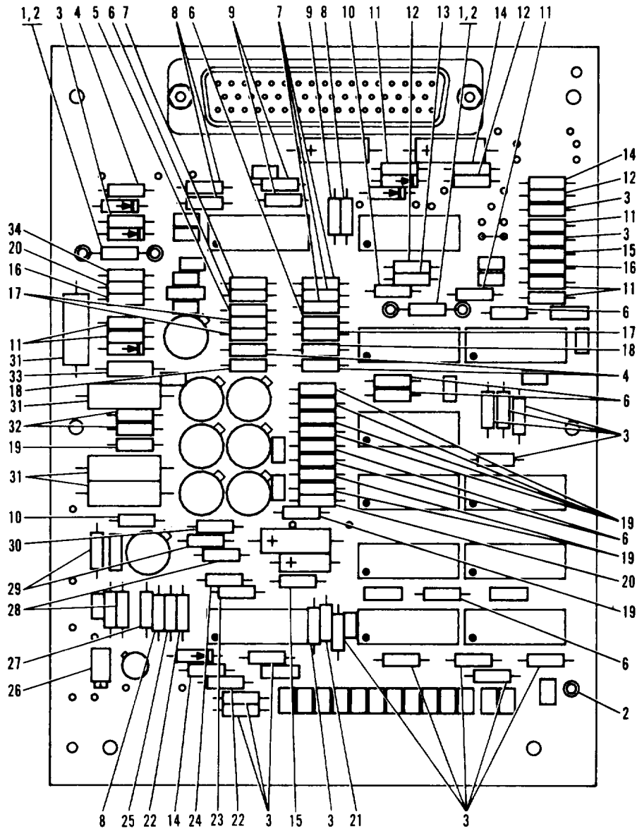
Figure 37. +40V Inverter/Driver Circuit Card subassembly (Sheet 1 of 2)
