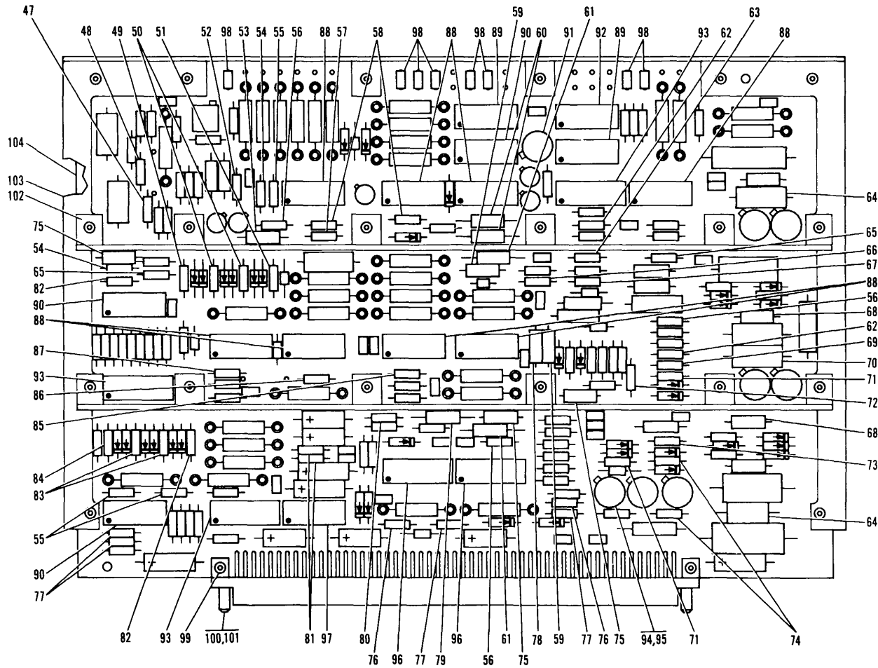
Figure 13. Type 6CFL Circuit Card Assembly (Sheet 3 of 3)
