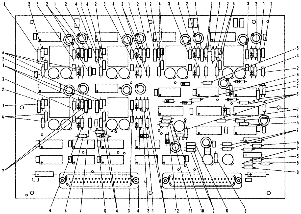
Figure 33. 3-Phase Inverter Circuit Card Subassembly (Sheet 1 of 3)
