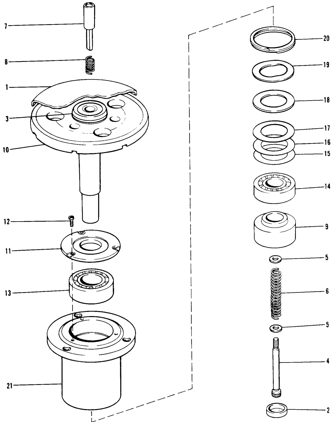
Figure 25. Spindle Assembly
