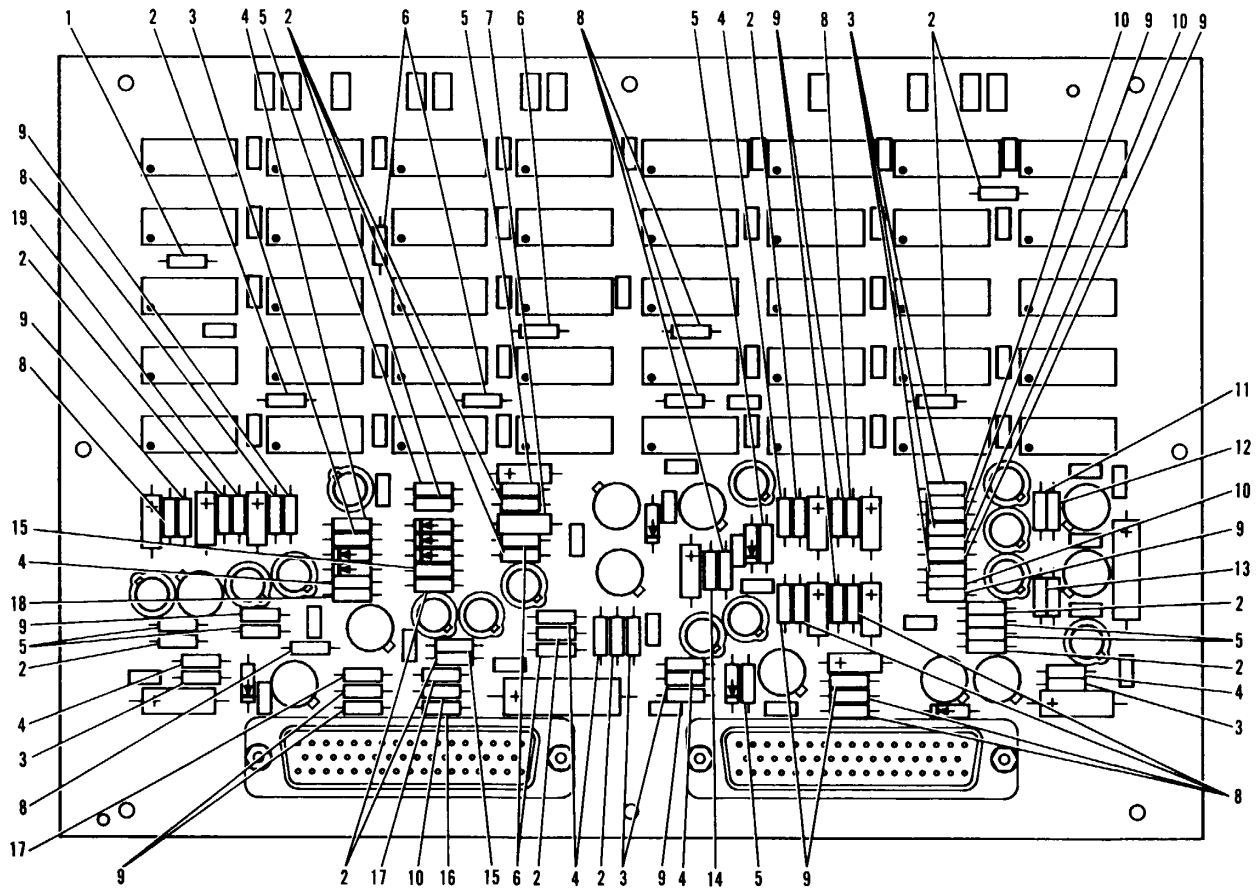
Figure 49. Power Control Circuit Card Subassembly (Sheet 1 of 3)
